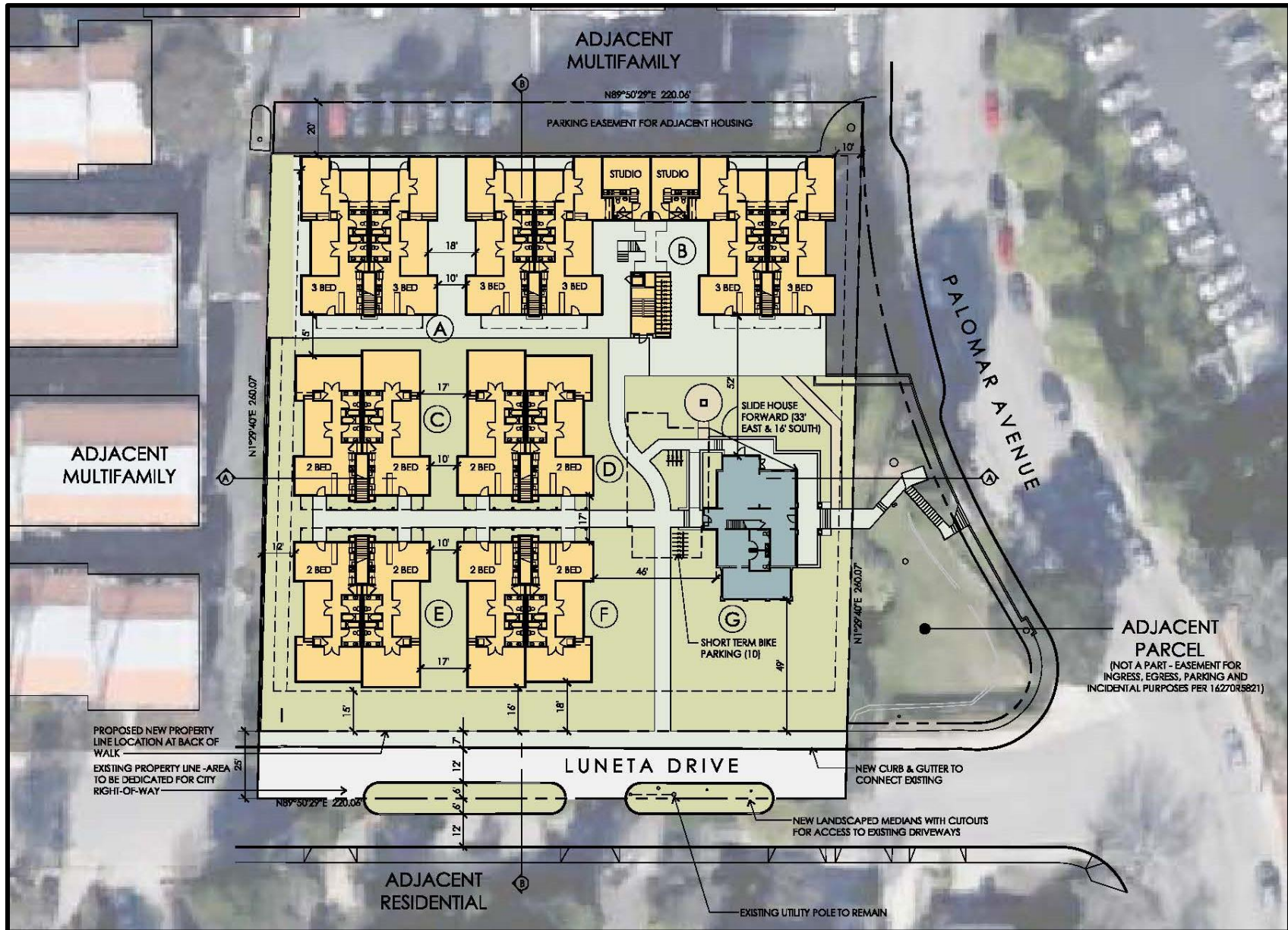
71 Palomar Avenue Multi-Family Residential Development City of San Luis Obispo
