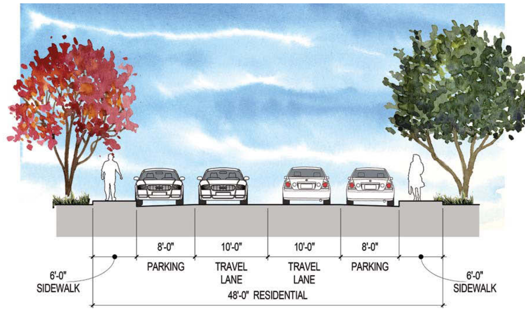
STREET SECTION
