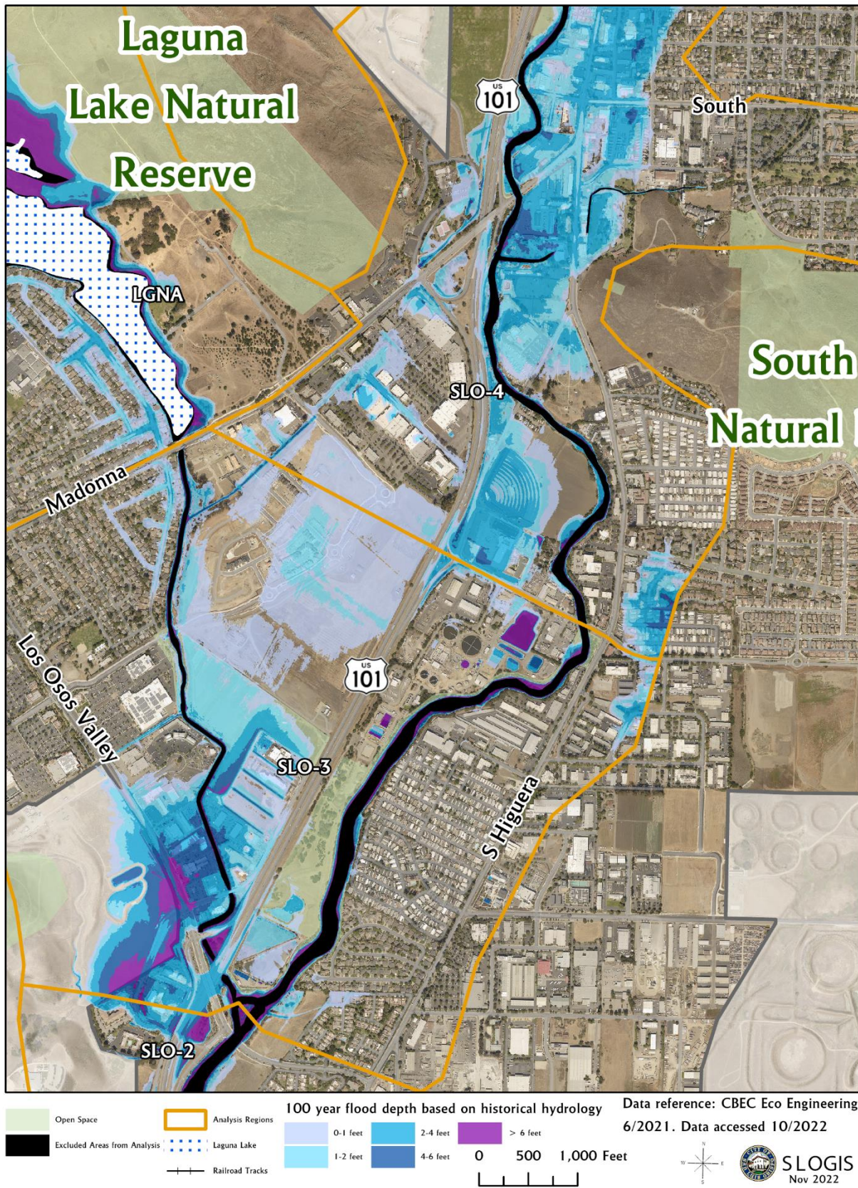
Figure 6 Flood depth: SLO Perfumo Historic (year 2000) Q100 event (1% chance of occurring in any given year) - based on historical hydrology
