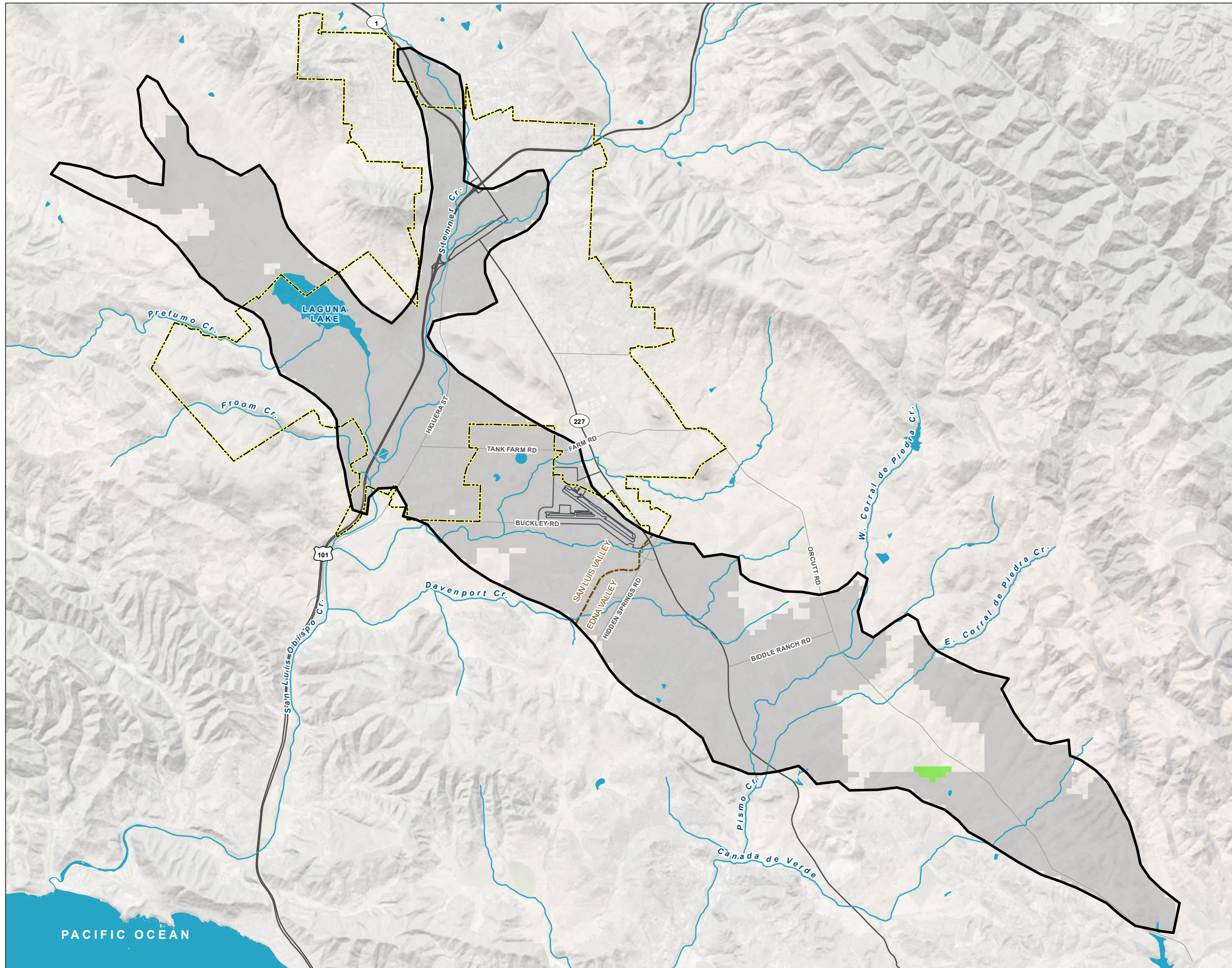
FIGURE 11 Five-Year Land Subsidence Measured by InSAR (June 2018-June 2023) San Luis Obispo, California
